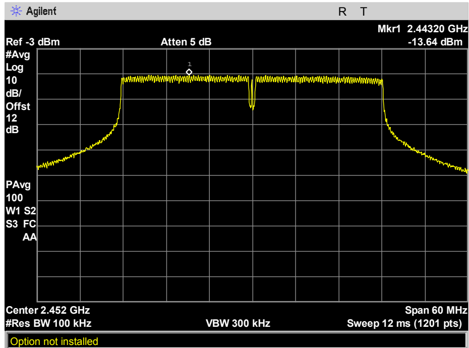
Plot 192. Power Density, 801.11n, 40, 2452, ch. 1
