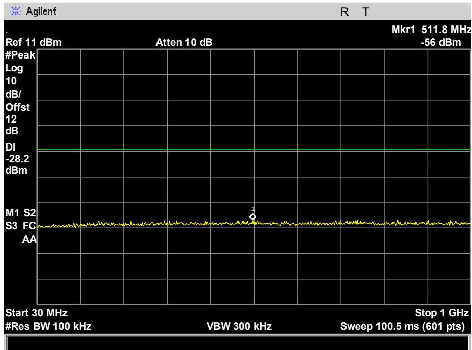
Plot 150. 100 kHz Spurious Emissions, 802.11g, 2412, 30 – 1000 MHz, ch 1
