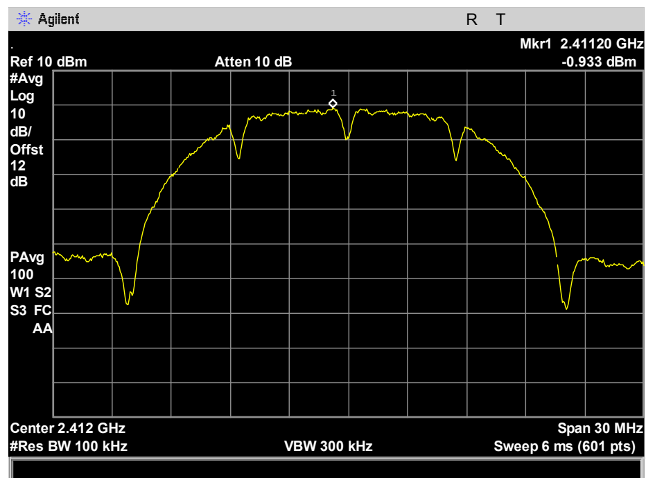
Plot 170. Power Density, 801.11b, 20, 2412, ch.1
