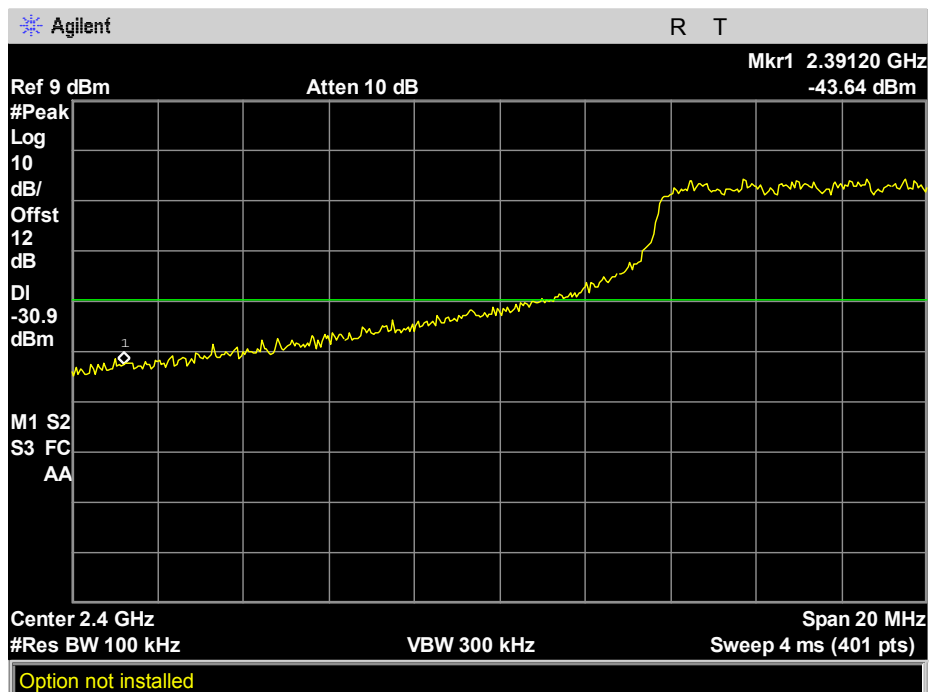
Plot 110. 100 kHz Spurious Emissions, 802.11n, 40M, 2422, Reference Level low bandedge, ch 1
