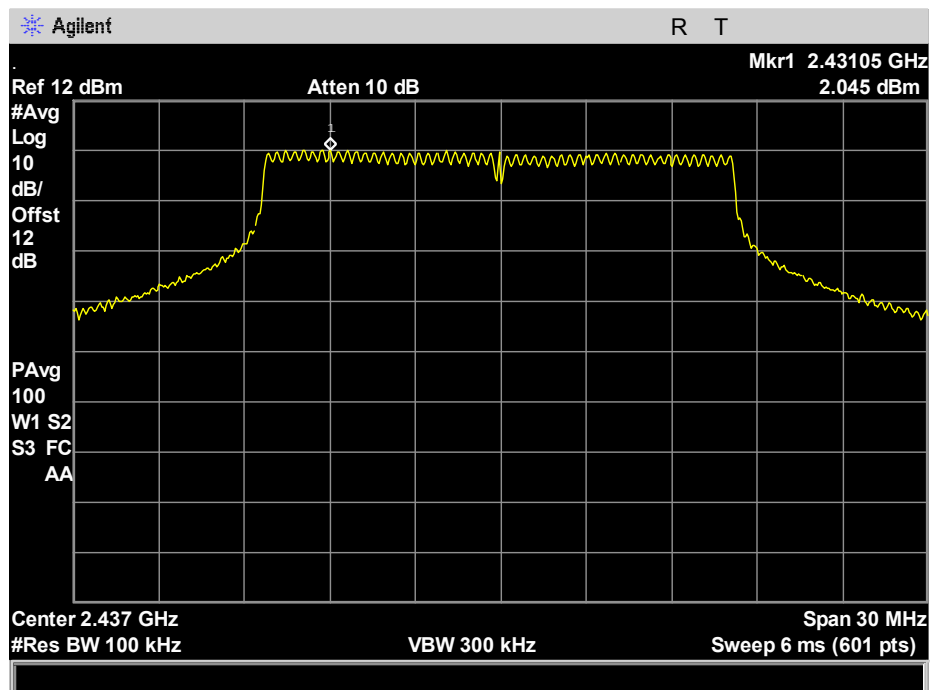
Plot 178. Power Density, 801.11g, 20, 2437, ch. 1
