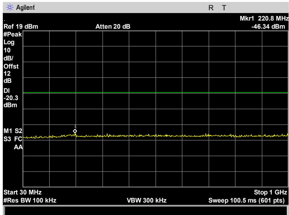
Plot 158. 100 kHz Spurious Emissions, 802.11g, 2437, 30 – 1000 MHz, ch 1
