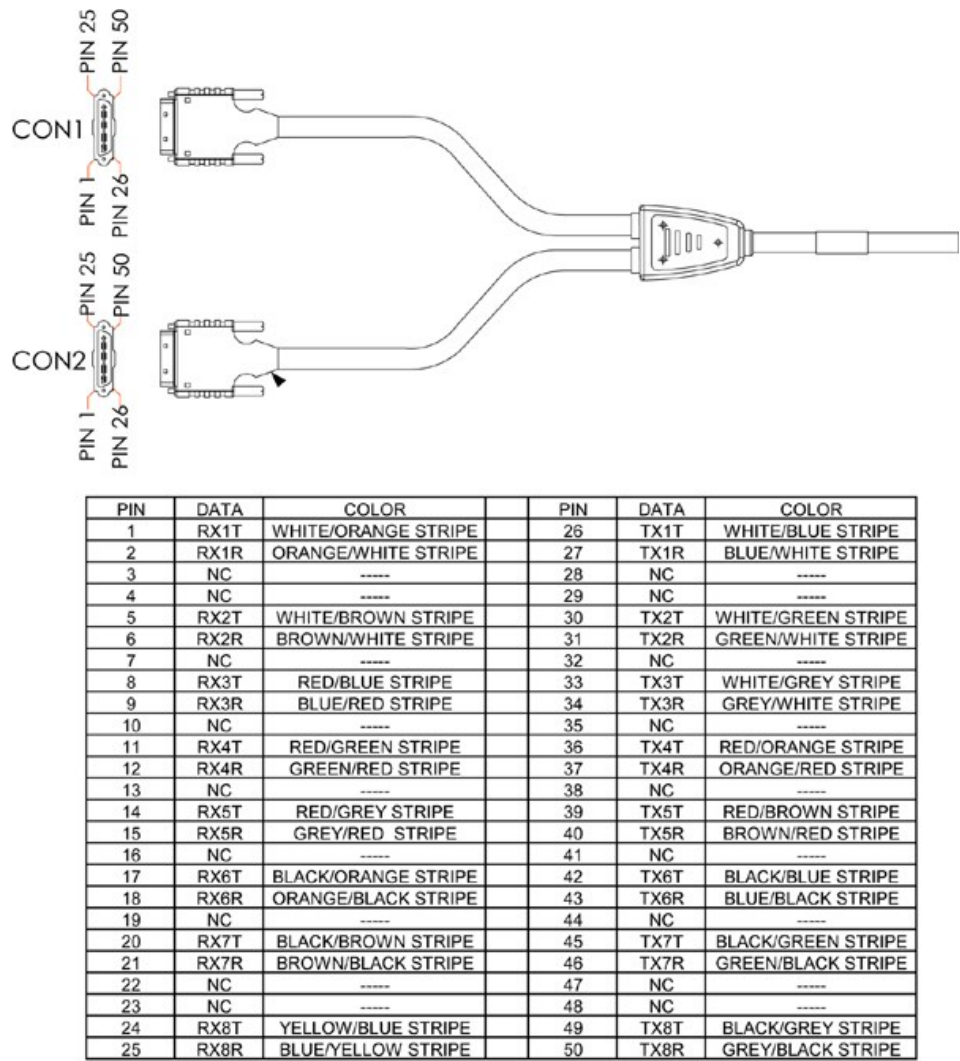
Figure 3-10. DAC 16xV2 Free End Y-Cable
