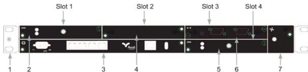
Figure 3-1. Typical INU Front Panel Layout
