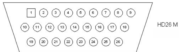
Figure 3-21. AUX TO AUX, HD26, 1M, ASYNC, Front View
