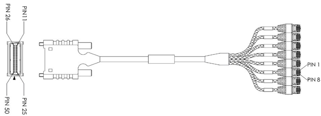
Figure 3-9. DAC 16xV2 RJ-45 Trib Cable Connections
