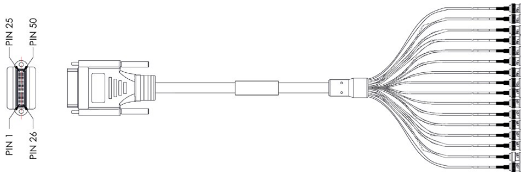
Figure 3-7. DAC 16xV2 BNC Trib Cable Connections
