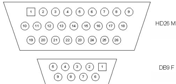
Figure 3-19. AUX HD26 and 3 X DB9, 1M, Async: Front Views
