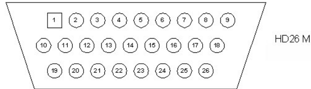
Figure 3-22. AUX TO AUX, HD26, 1m, Sync, Front View
