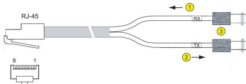
Figure 3-13. DAC 4x RJ-45 to BNC Cable
