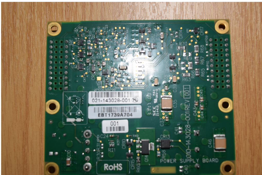
Photo 6, IRU 600v4 DC power board side 1:
