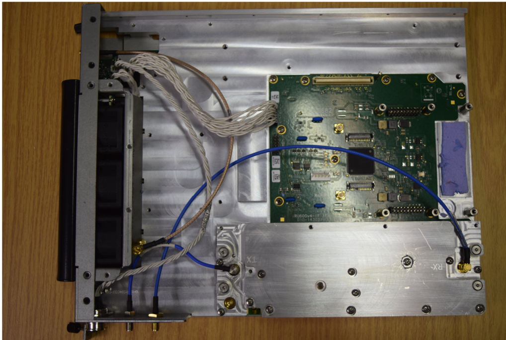
Photo 5, IRU 600v4 RFU close up, DC power board removed:
