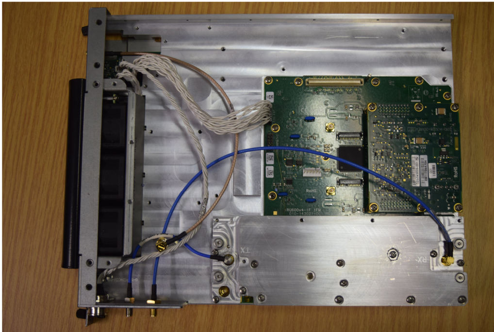
Photo 3, IRU 600v4 RFU lid removed close up:
