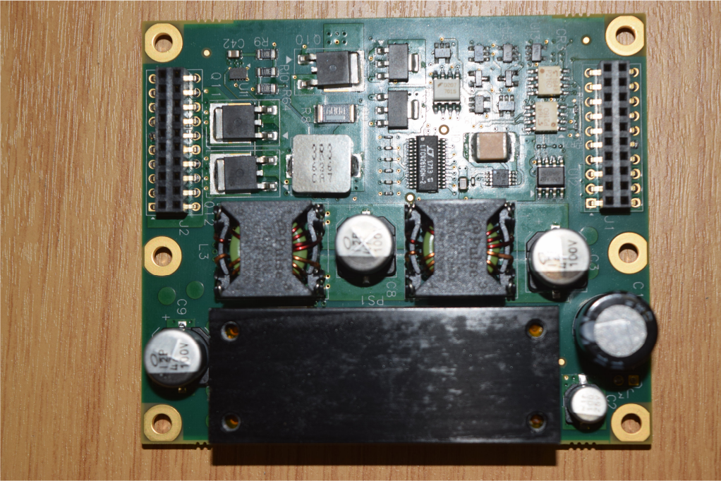
Photo 7, IRU 600v4 DC power board side 2:
