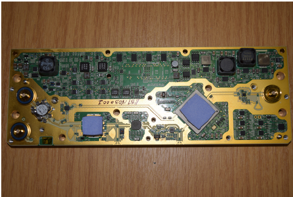
Photo 10, IRU 600v4 transceiver side 2 shield removed:
