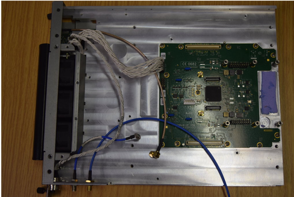
Photo 11, IRU 600v4 RFU close up, transceiver removed:
