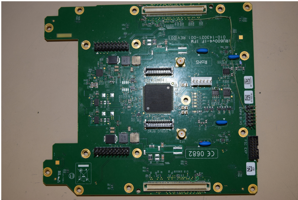
Photo 13, IRU 600v4 IFM card side 1:
