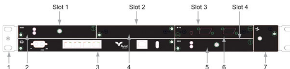
Figure 42. Typical INU Front Panel Layout
