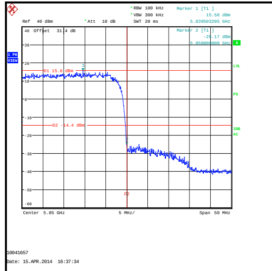
Upper Band Edge Peak Measurement – 128QAM
