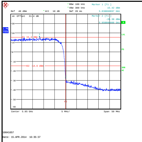
Upper Band Edge Peak Measurement – 64QAM
