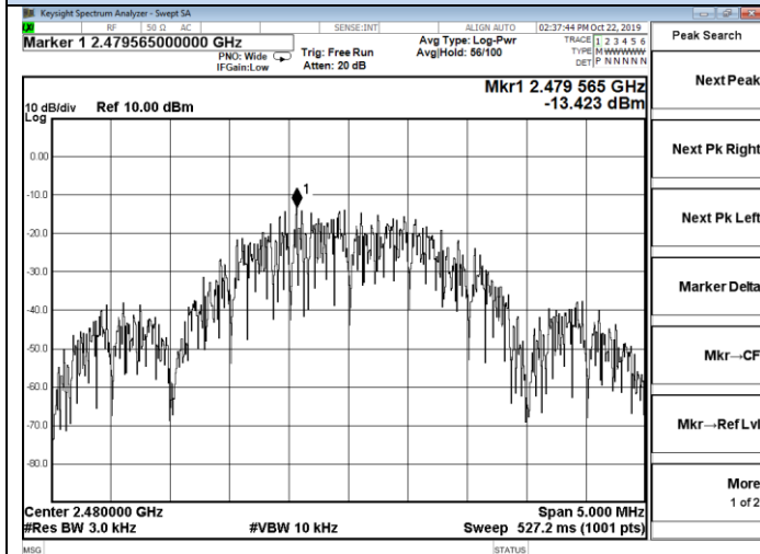
Channel 15 / 2480 MHz
