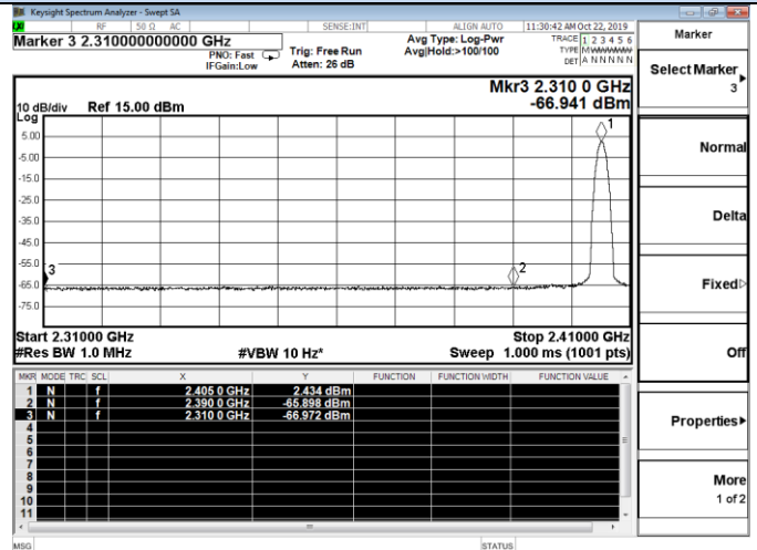
Channel 0 / 2405 MHz – Average
