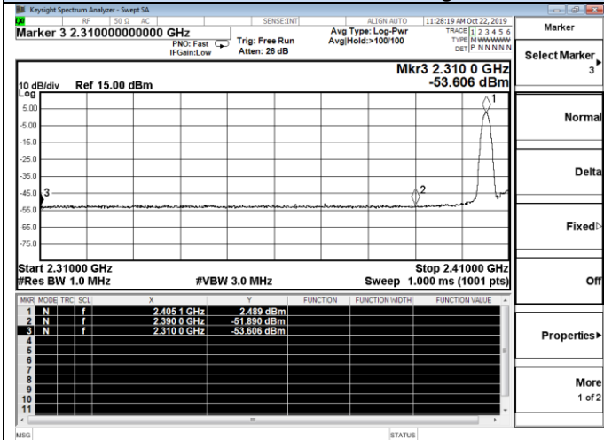
Channel 0 / 2405 MHz – Peak
