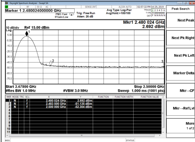
Channel 15 / 2480 MHz – Peak
