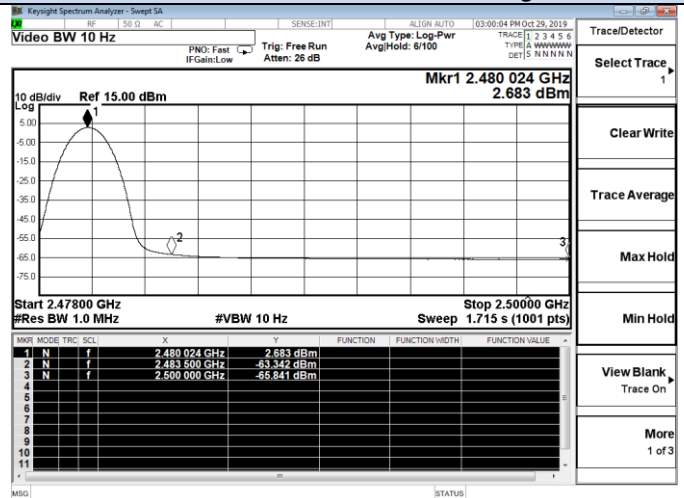
Channel 15 / 2480 MHz – Average
