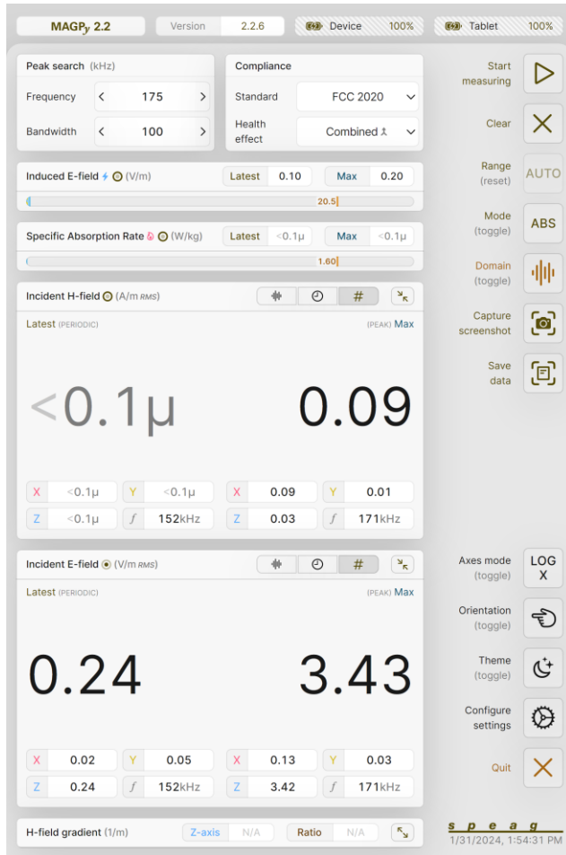
Wireless Power Transfer (WPT) d(\text{enc}) = 6 \text{ cm} Numeric display
