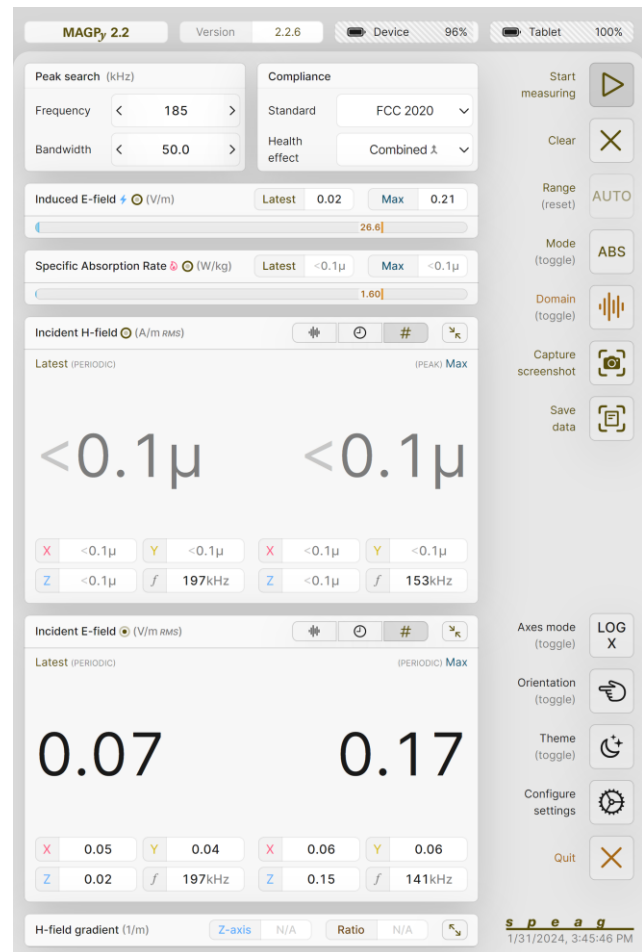
Wireless Power Transfer (WPT) d(enc) = 20 cm Numeric display
