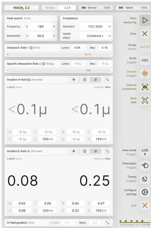
Wireless Power Transfer (WPT) d(enc) = 18 cm Numeric display
