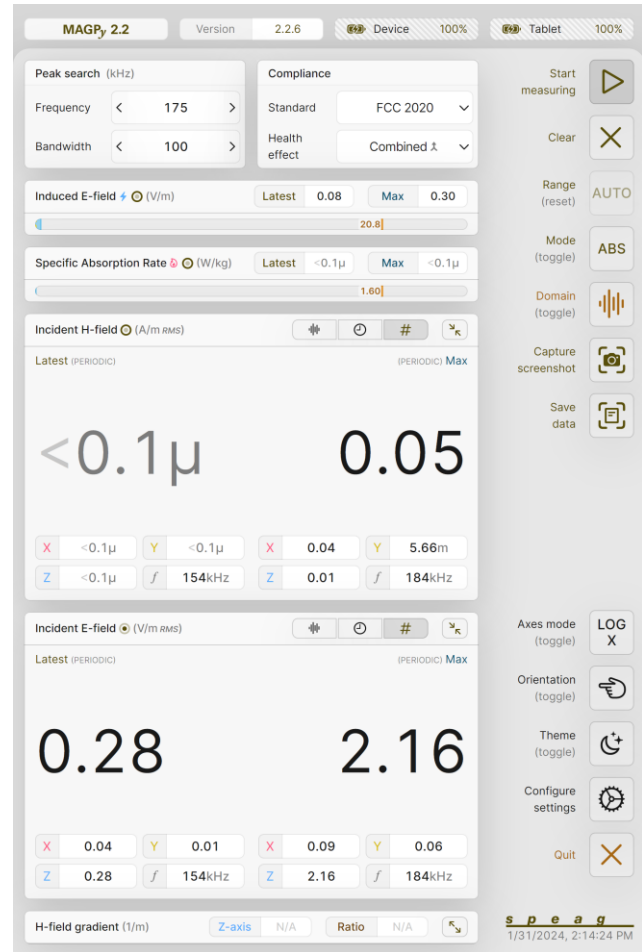
Wireless Power Transfer (WPT) d(\text{enc}) = 8 \text{ cm} Numeric display
