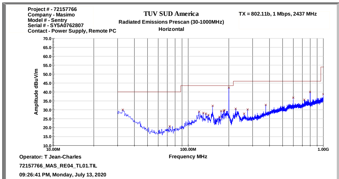
Figure 2.2.7-2: Radiated Emissions Representative Scan 30 MHz – 1 GHz – Horizontal Polarization – Wi-Fi
