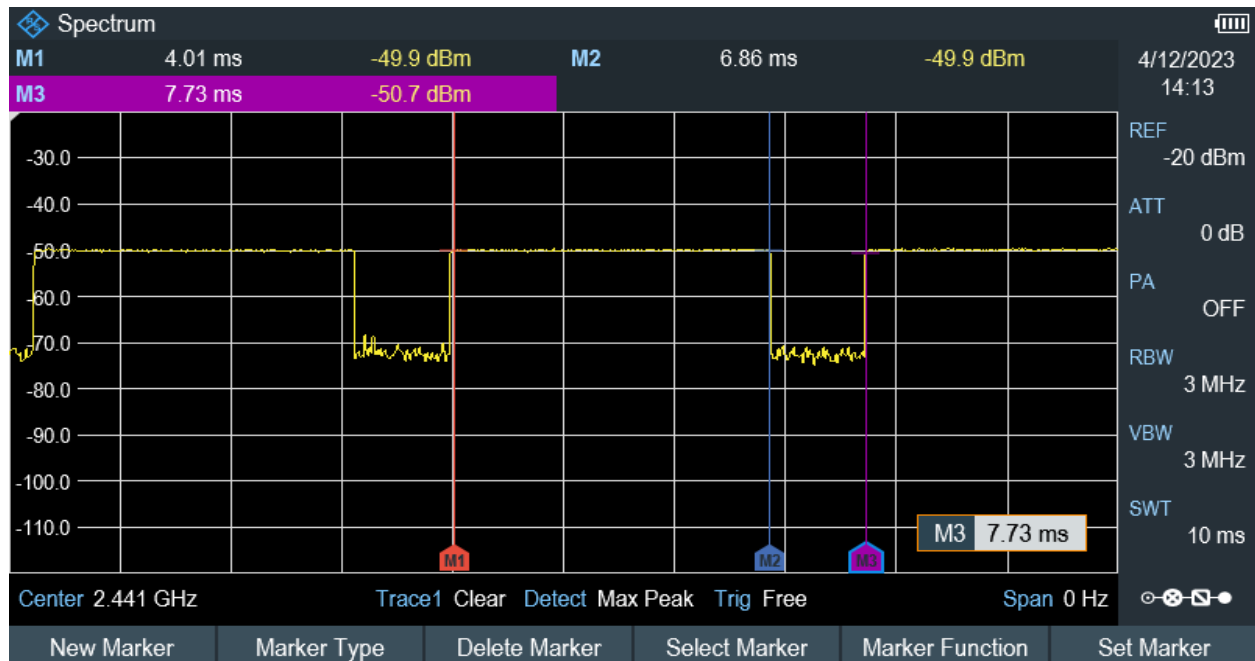
Time-domain plot for Bluetooth transmission signal
