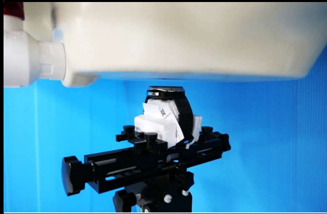
Front Face of EUT Tested at 10 mm for WWAN / WLAN / BT
