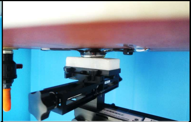
Rear Face of EUT Tested at 0 mm for NFC
