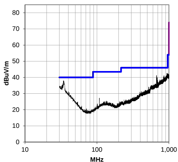
30-1000 MHz, Run 29
