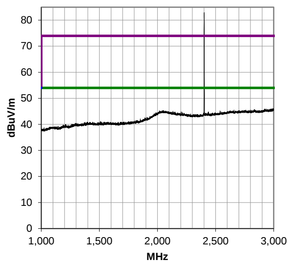
1000-3000 MHz, Run 34
