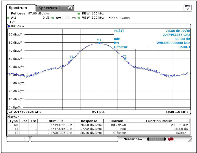
Bandwidth 3 (2475MHz)
