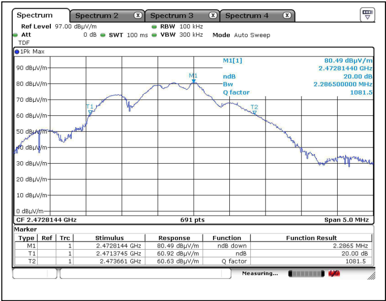
Bandwidth 3 (2472MHz)
