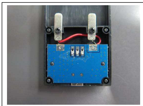
Internal Configuration 10
