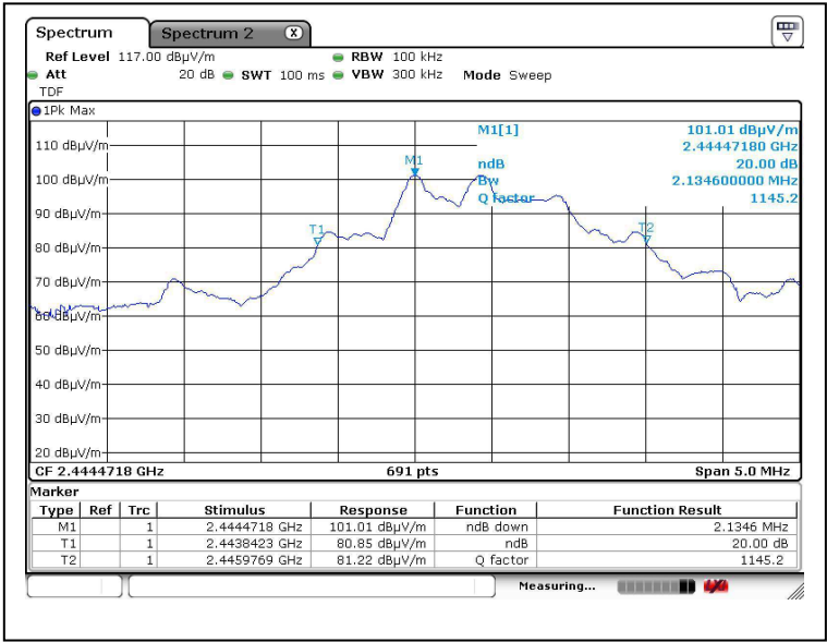
Bandwidth 2 (2445MHz)
