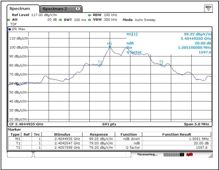
Bandwidth 1 (2405MHz)
