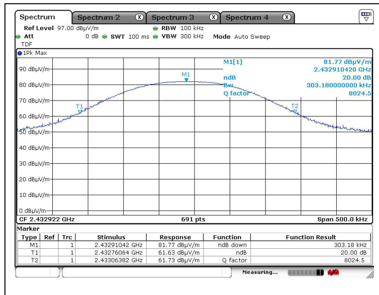
Bandwidth 2 (2433MHz)
