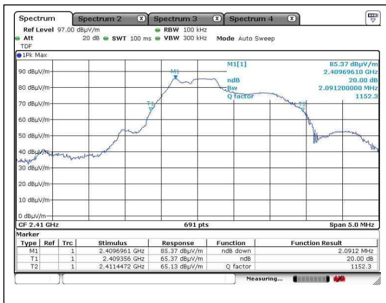
Bandwidth 1 (2410MHz)
