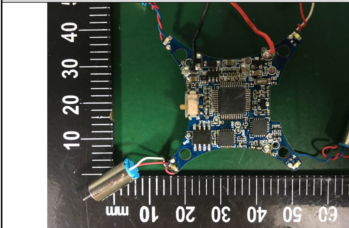
EUT Photo #8 PCB View
