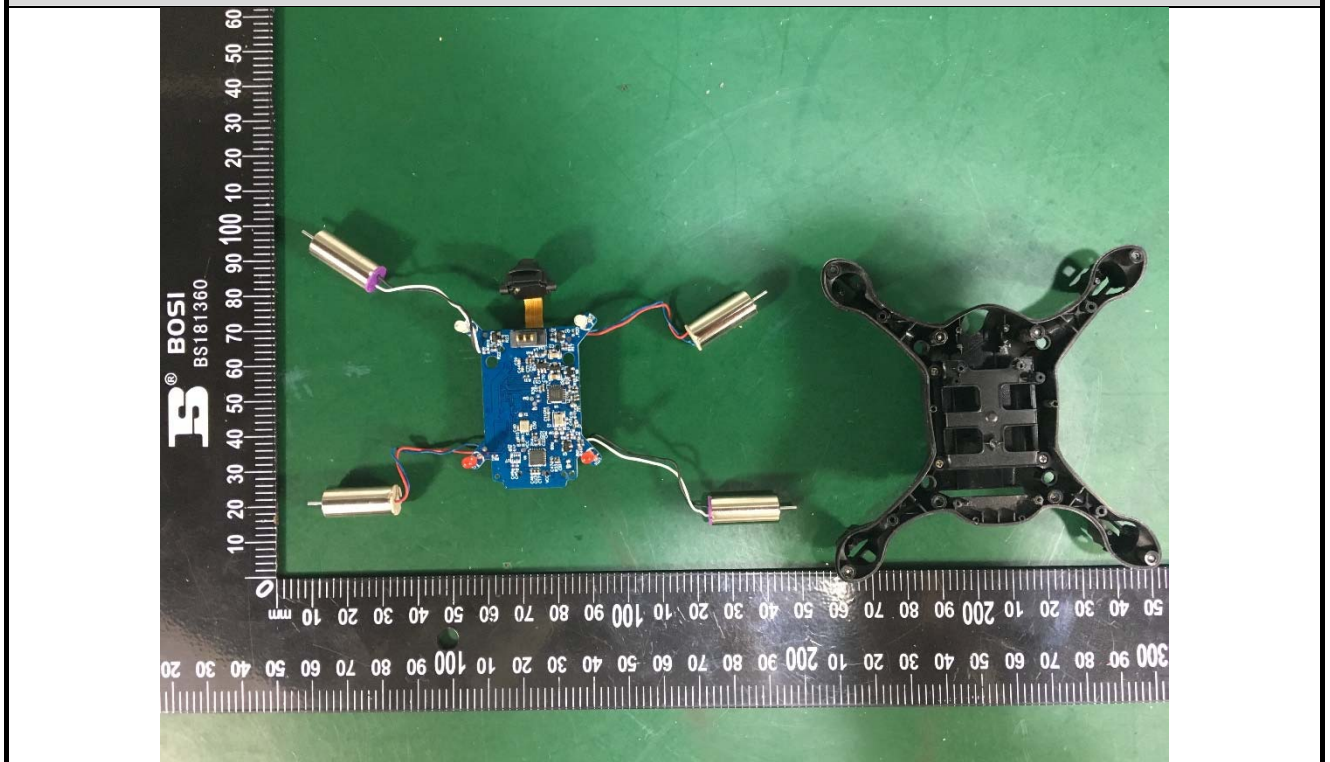
EUT Photo #2 Uncover View
