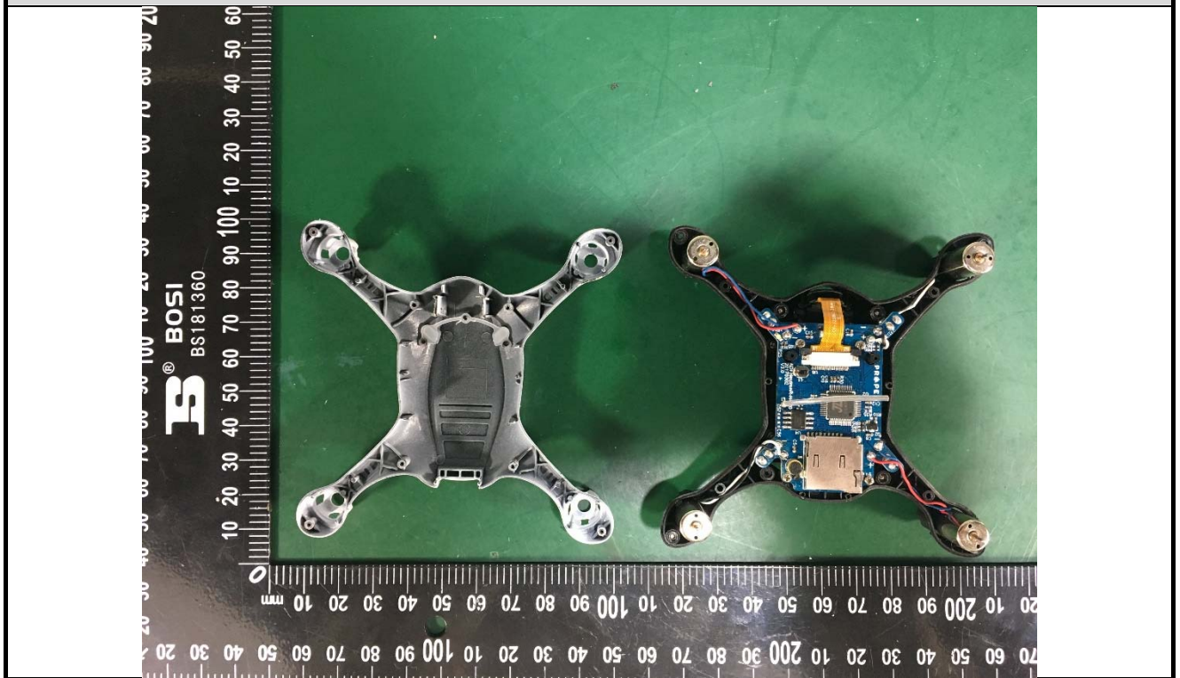
EUT Photo #1 Uncover View
