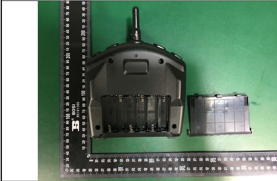
EUT Photo #1 Uncover View
