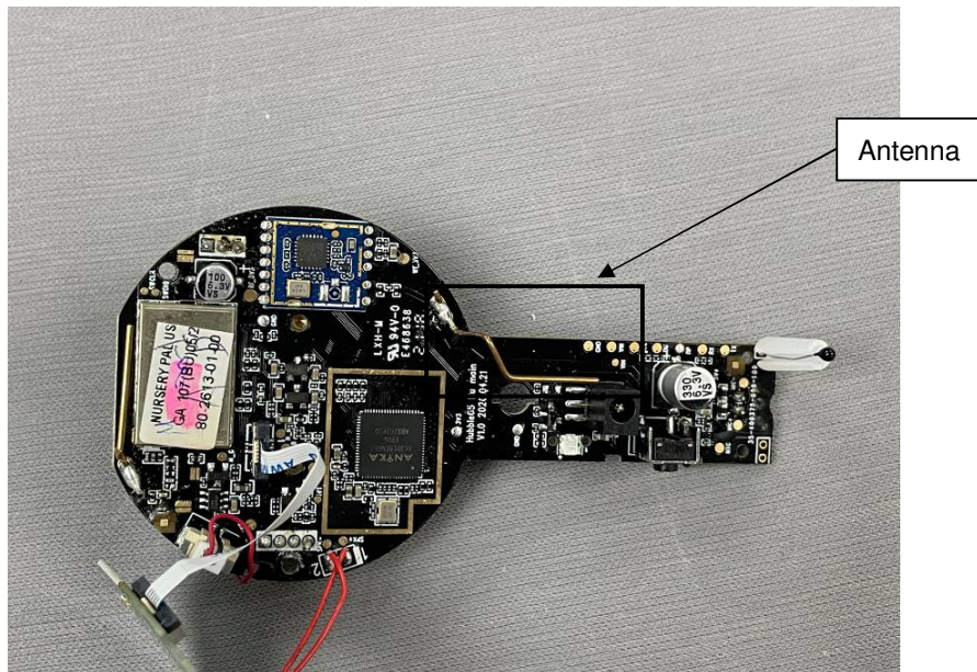
Photo of antenna refer to Appendix – Internal photo.
