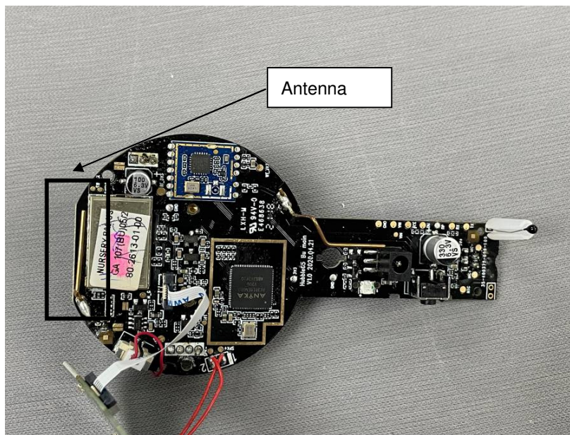
Photo of antenna refer to Appendix – Internal photo.
