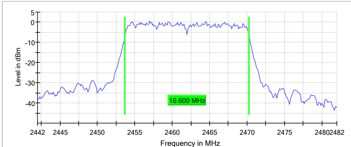
99 % Bandwidth
