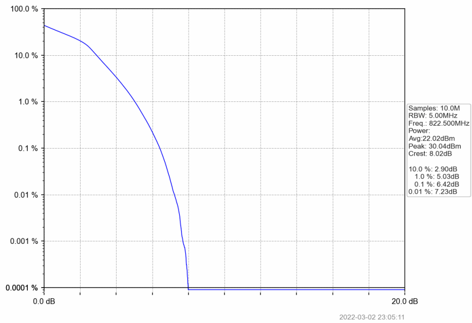
Band26a 3MHz 16QAM HCH 822.5MHz RB 15 0 NTNV
