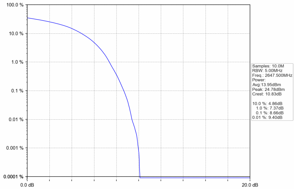
Band41 15MHz QPSK HCH 2647.5MHz RB 75 0 NTN
