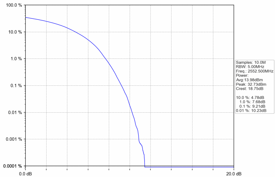
Band41 15MHz 16QAM LCH 2552.5MHz RB 75 0 NTN
