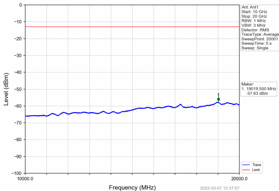
Band2_RMC_MCH_1880MHz_12.2kbps RMC_NTNV
