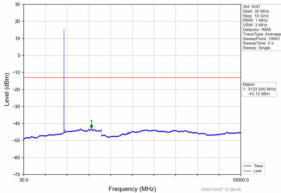
Band2_RMC_MCH_1880MHz_12.2kbps RMC_NTNV
