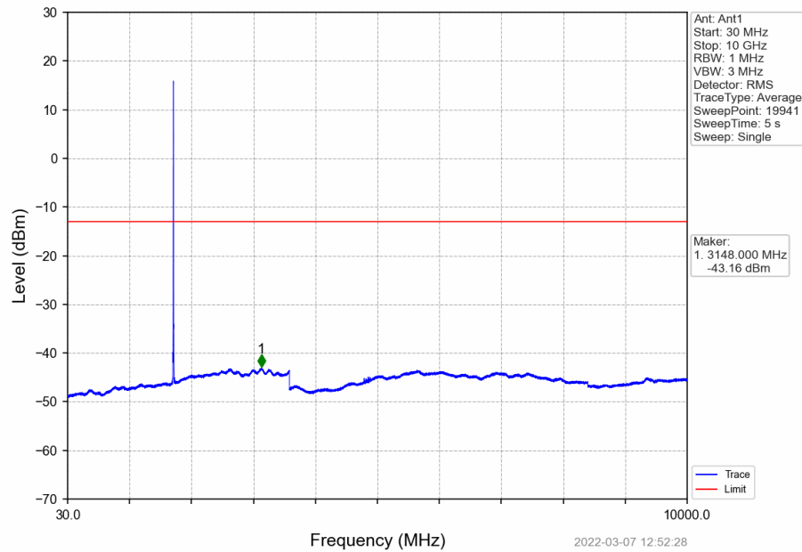
Band4_HSUPA_MCH_1732.6MHz_Subtest 1_NTNV
