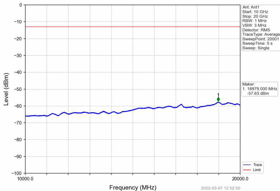
Band4_HSUPA_MCH_1732.6MHz_Subtest 1_NTNV
