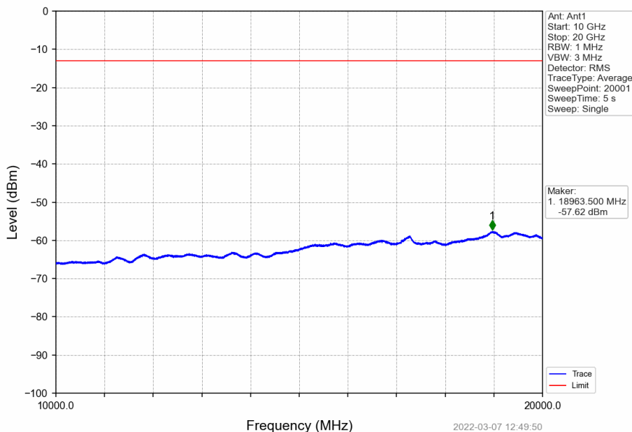
Band4_HSDPA_MCH_1732.6MHz_Subtest 1_NTNV
