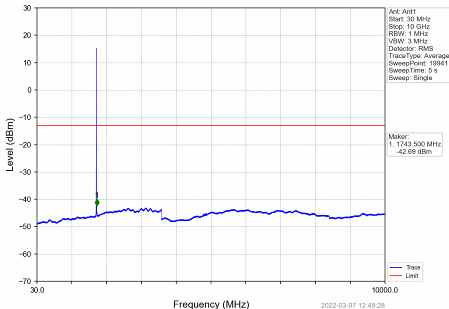
Band4_HSDPA_MCH_1732.6MHz_Subtest 1_NTNV
