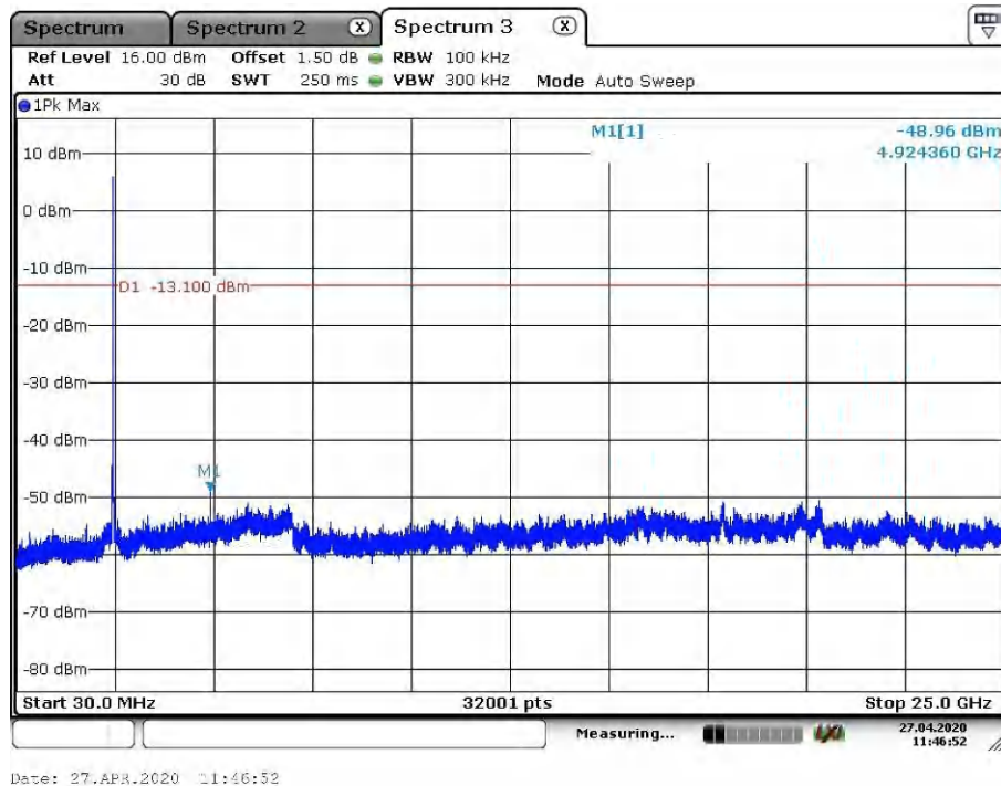
Wi-Fi 802.11 g mode, 6 Mbps
