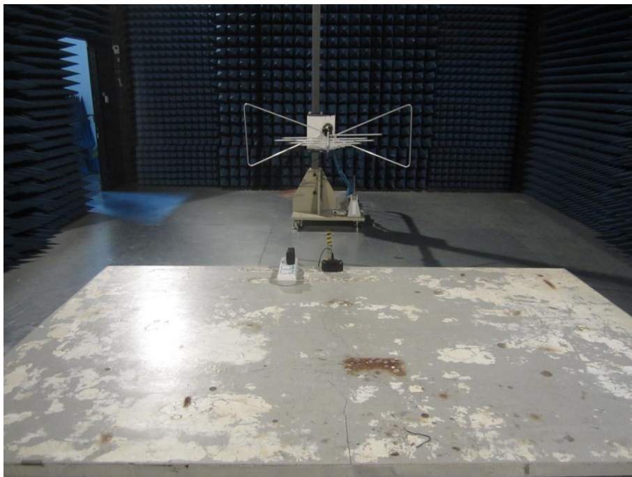
Figure 2 Setup for Radiated Emission(below 1GHz)
