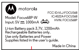
Rating Label Size:35.5X22mm White background black letters
