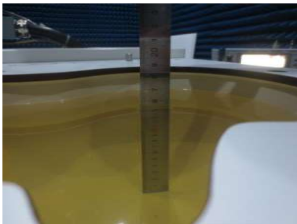
Fig. 9.1 Photo of Liquid Height for Head SAR (1900MHz) (depth>15cm)
