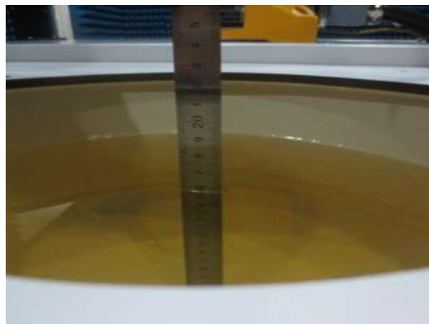
Fig. 9.2 Photo of Liquid Height for Body SAR of Twin Phantom (1900MHz) (depth>15cm)
