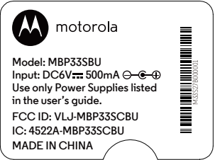
Rating Label(BU) Material: 50# PET Size : 39.5 x 29.5 mm
