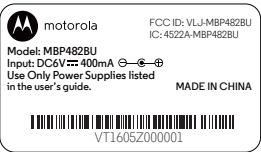
Rating Label(BU) Material: 50# PET Size : 34.5x19.6mm
