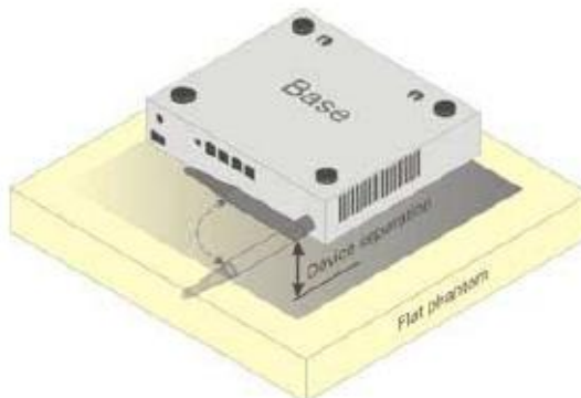
Figure 6 – Device with swivel antenna (example of desktop device)
