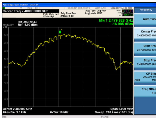
LE-1Mbps CH39 (2480MHz)
