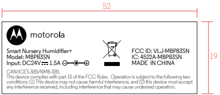
MBP83SN Rating Label (for North America)
