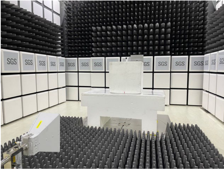
Radiated Emissions (Above 1GHz) Test Setup
