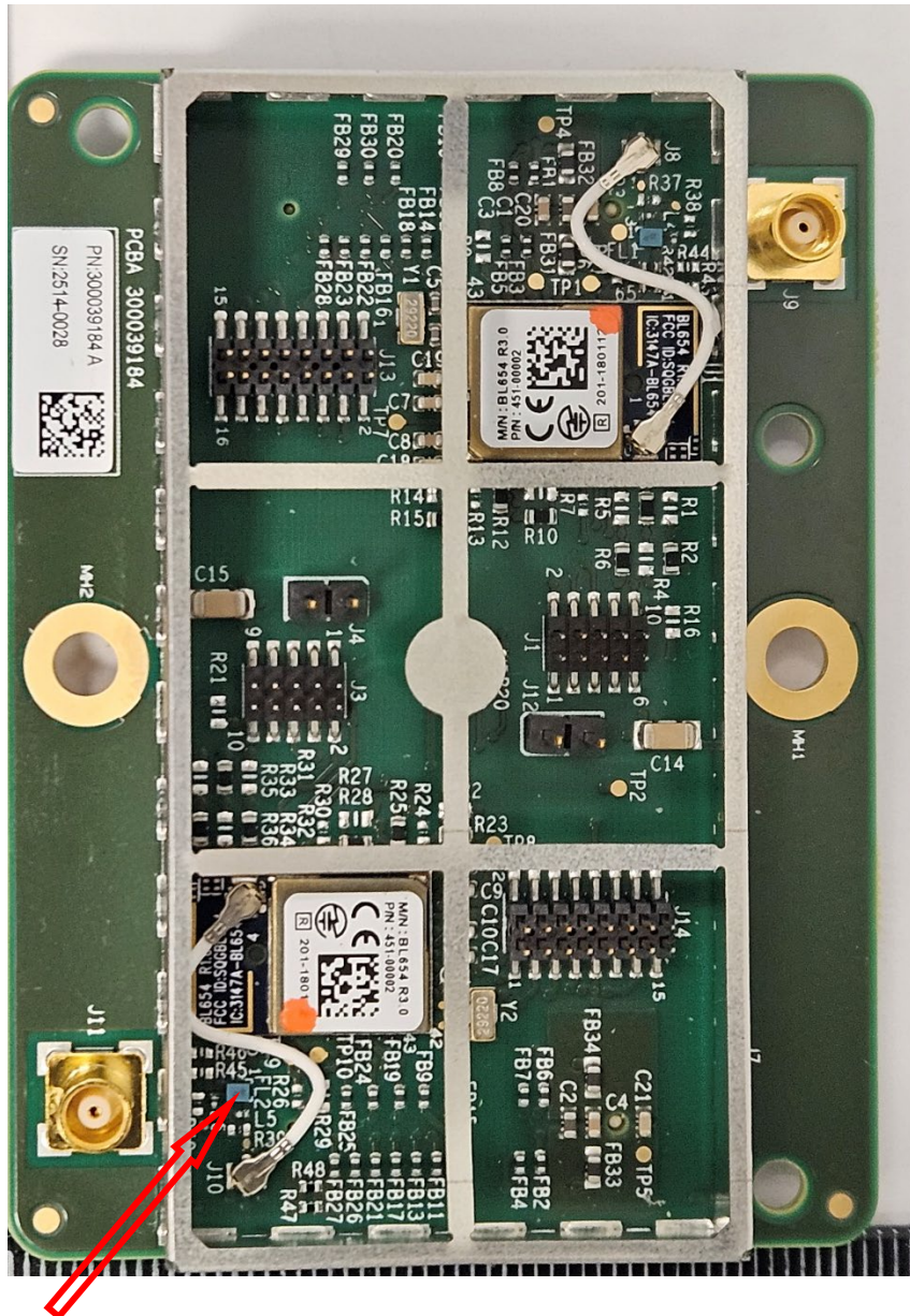
Bandpass Filter
