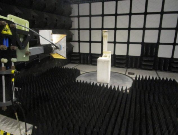
200-1000 MHz
