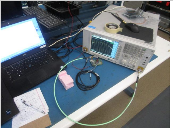
Conducted RF Bench
