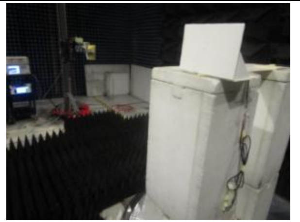
1-4 GHz
