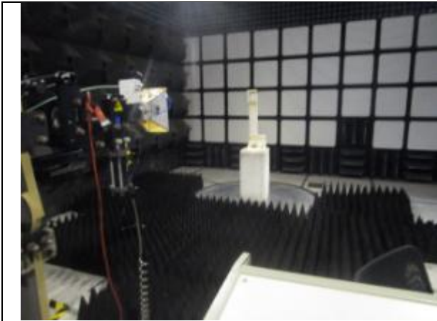
4-18 GHz
