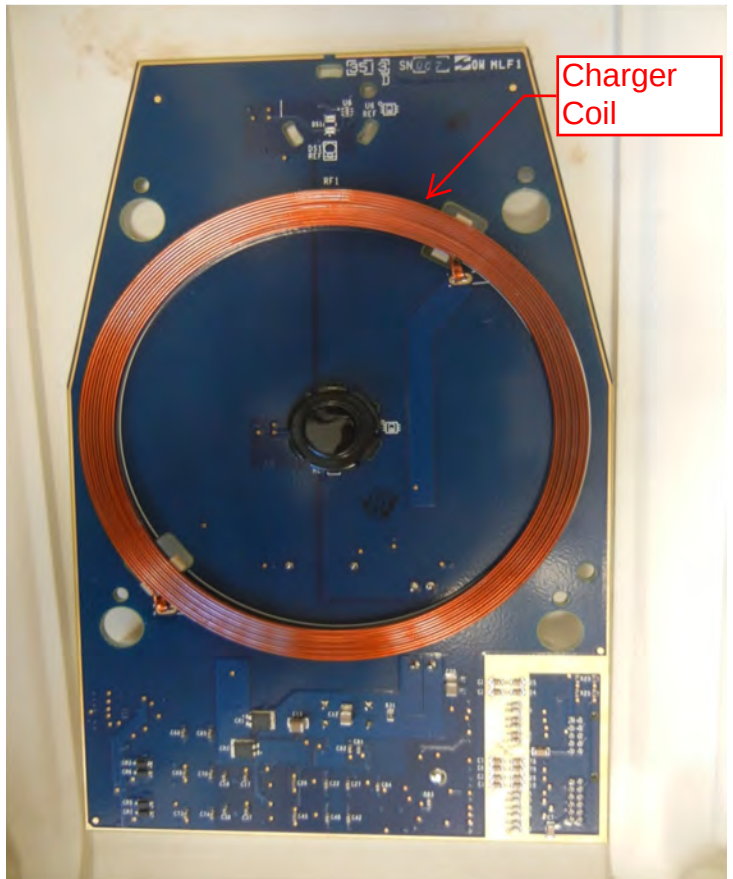
Charger Coil PCB, LuxOR Microscope Side – bottom view
