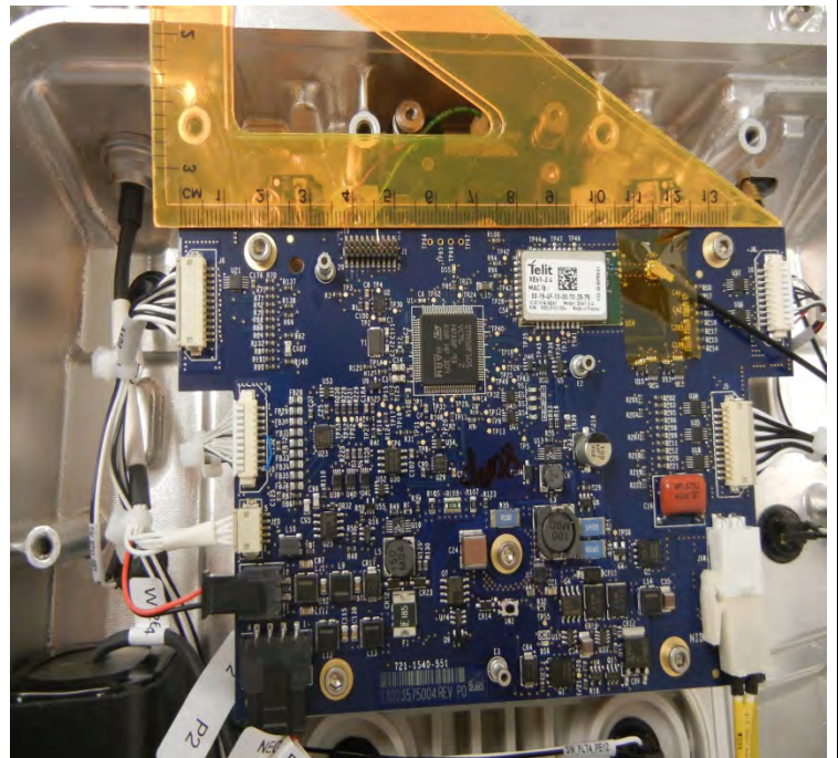
Receiver Coil PCB (Foot Controller Side)
