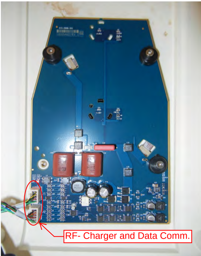
Charger Coil PCB, LuxOR Microscope Side – top view
