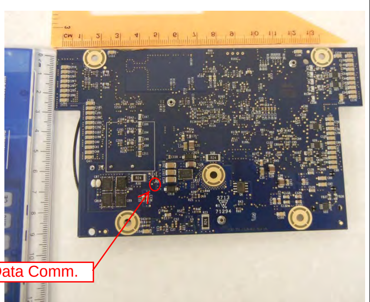
Receiver Coil PCB (Foot Controller Side – bottom view)
