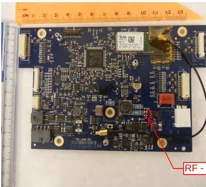
Receiver Coil PCB (Foot Controller Side – top view)
