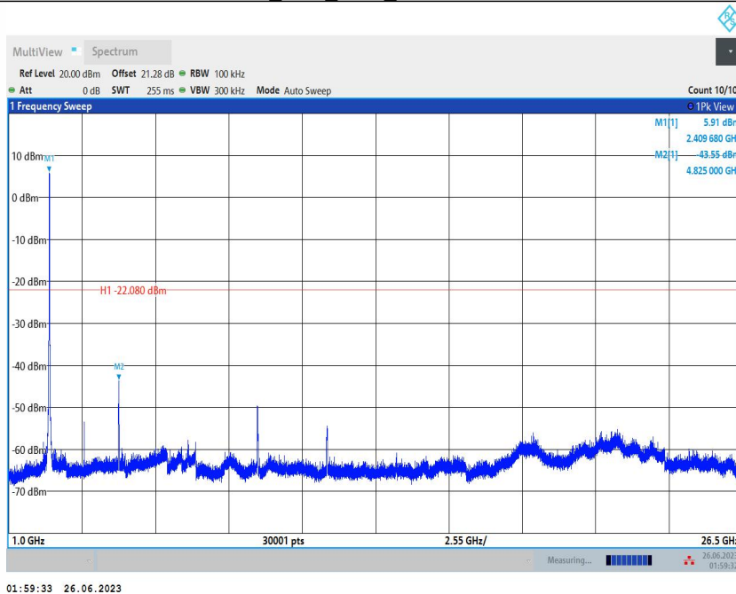
11G_Ant1_2437_0~Reference
