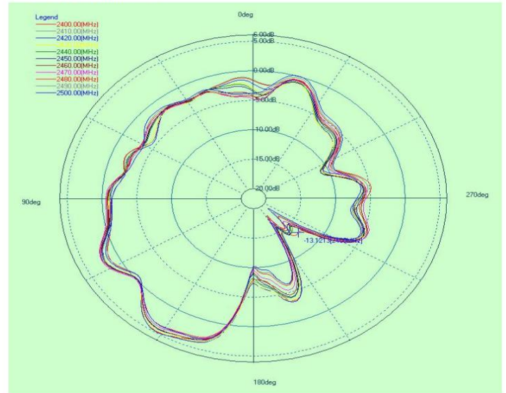
H-Plane (Elevation 90° )
