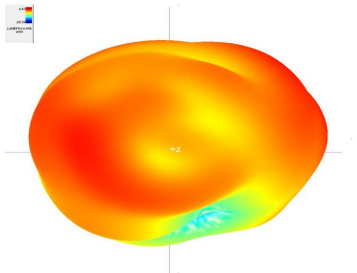
3D view Frequency 2450MHz
