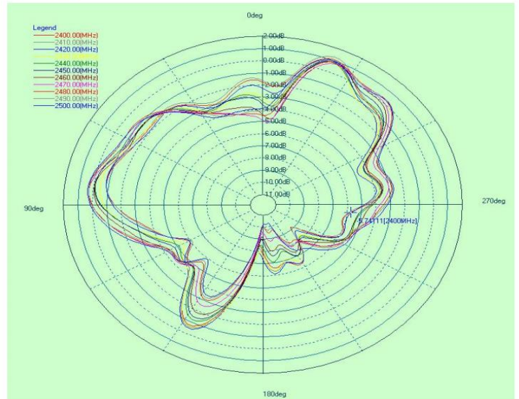
Azimuth 0°
