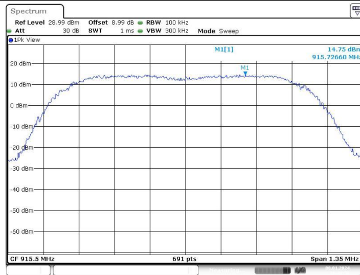
WiFi HaLow (1Mbps)_Ant1_915.5
