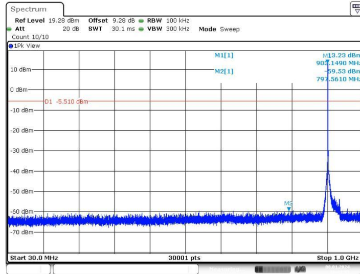
WiFi HaLow (1Mbps)_Ant1_903.5_30~1000
