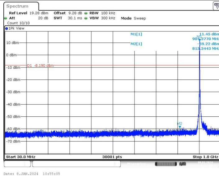
WiFi HaLow (2Mbps)_Ant1_905_1000~26500
