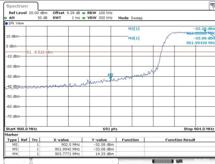
WiFi HaLow (1Mbps)_Ant1_Low_903.5
