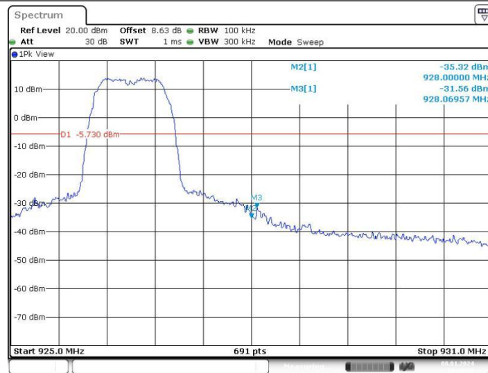
WiFi HaLow (1Mbps)_Ant1_High_926.5
