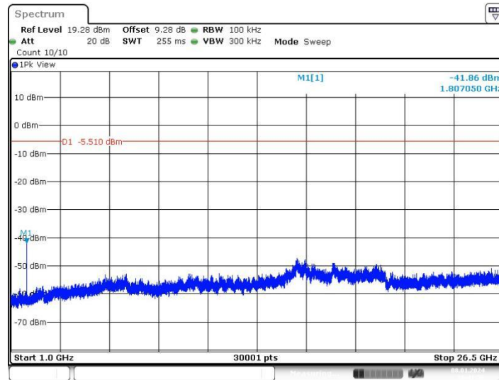
WiFi HaLow (1Mbps)_Ant1_903.5_1000~26500
