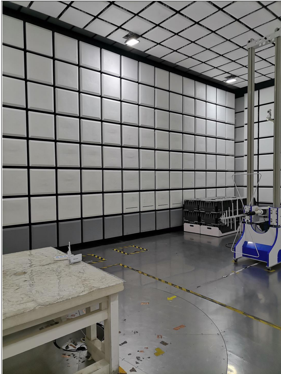
RADIATED EMISSION TEST (Below 1GHz)
