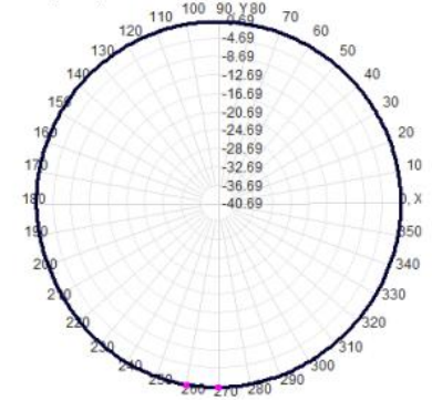
Total(H-XY), Max=-0.72dBi, CirD=0.59
