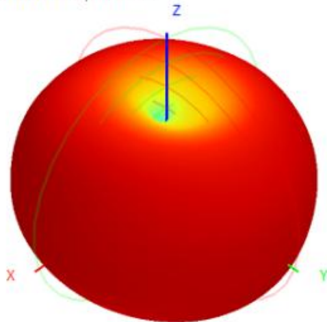
915.0MHz H+V, Eff: 59.2%
