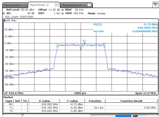
4M-Middle channel
