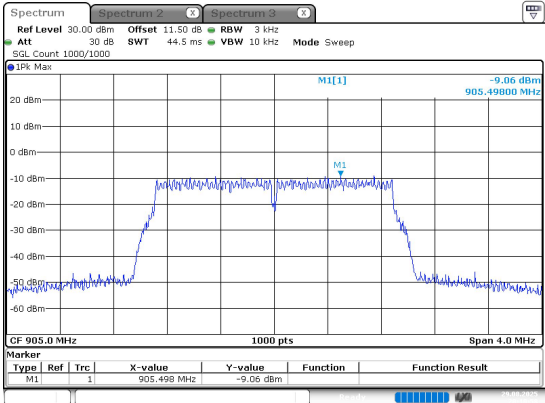
2M-Low channel
