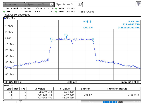
4M-High channel
