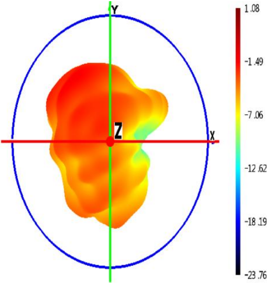
915MHz 3D_Graphs
