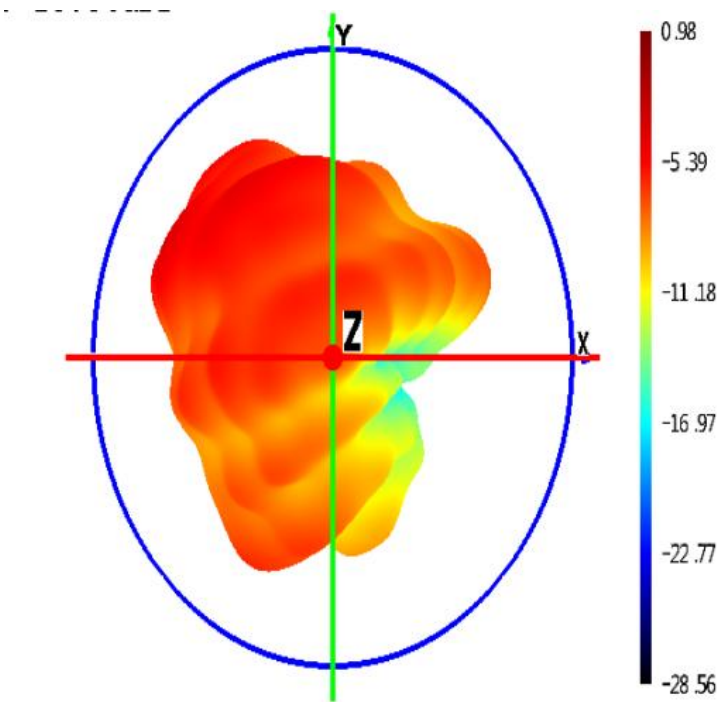
433.92MHz 3D_Graphs
