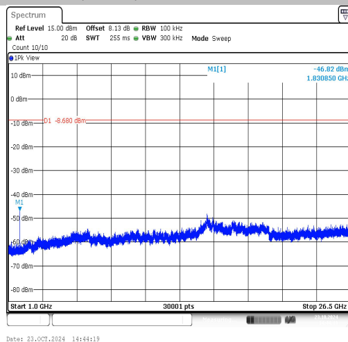
WiFi HaLow (1Mbps)-Ant1-915.5-1000~26500-PASS
