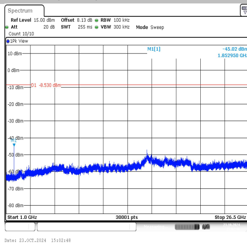
WiFi HaLow (1Mbps)-Ant1-926.5-1000~26500-PASS
