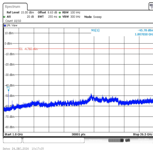
WiFi HaLow (1Mbps)-Ant1-903.5-1000~26500-PASS
