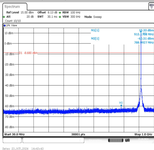
WiFi HaLow (1Mbps)-Ant1-915.5-30~1000-PASS
