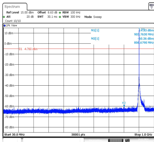
WiFi HaLow (1Mbps)-Ant1-903.5-30~1000-PASS
