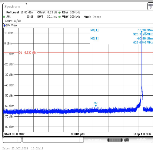
WiFi HaLow (1Mbps)-Ant1-926.5-30~1000-PASS
